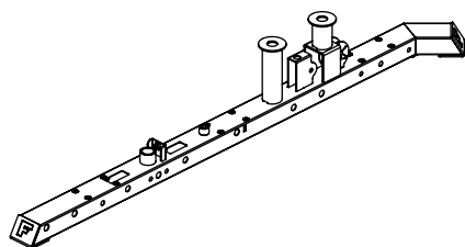
Base Frame - Right
