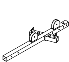
(1) MAIN FRAME
